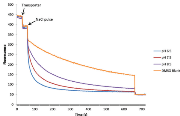
Fig. 8 Chloride influx promoted by 0.05 mol% of ester 3f as a function of pH. At t = 20 s a solution of 3f was added to a solution of EYPC vesicles ( d = 200 nm), loaded with 100 mM NaNO 3 and suspended in 10 mM phosphate buffer (pH 6.5, 7.5 or 8.5). At t = 60 s NaCl solution was added to give a final extravesicular Cl - concentration of 100 mM. At the end of the experiment, Triton detergent was added to lyse the vesicles. The faster fluorescence decay indicates faster anion exchange, as mediated by ester 3f .
