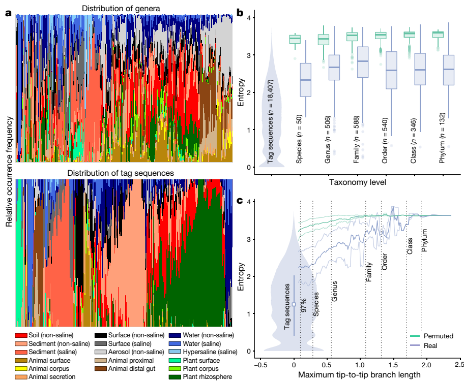
Figure 4 | Specificity of sequences and higher taxonomic groups for environment. a , Environment distribution in all genera and 400 randomly chosen tag sequences, drawn from n = 2,000 biologically independent samples with even representation across environments (EMPO level 3) and studies. Each bar depicts the distribution of environments for a taxon (not relative abundance of taxa): bars composed mostly of one colour (environment) are specific for that environment, as seen with tag sequences; bars composed of many colours are more cosmopolitan, as seen with genera. Tag sequences were more specific for environment than were genera and higher taxonomic levels. b , Shannon entropy within each taxonomic group (minimum 20 tag sequences per group) and for the same set of samples with permuted taxonomy labels. Box plots show
