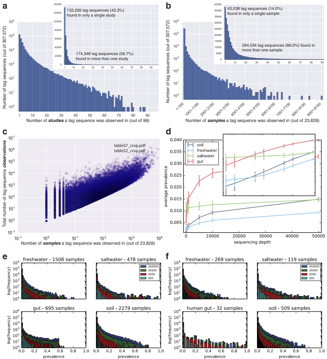
Extended Data Figure 4 | Tag sequence prevalence patterns. Note that for this meta-analysis, the input observation table was filtered to keep only tag sequences with at least 25 observations total over all samples and then rarefied to 5,000 observations per sample. a , Per-study endemism visualized as a histogram of tag sequences binned by the number of studies in which they are observed (left: linear scale; right: log scale). b , Per-sample endemism visualized as a histogram of tag sequences binned by the number of samples in which they are observed (left: sample counts up to 92 samples and the number of tag sequences in linear scale; right: all tag sequences with bin widths of 100 samples and number of tag sequences in log scale). c , Abundance (total observations in rarefied table) versus prevalence (number of samples observed in) of n = 307,572 tag sequences. Both axes are log scale. The most prevalent tag sequences were also the most abundant. d , Prevalence as a function of sequencing
